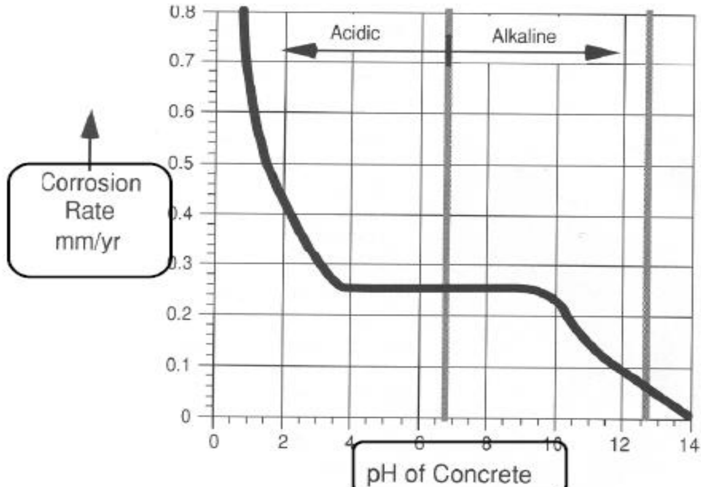
Relationship between pH and corrosion rate
